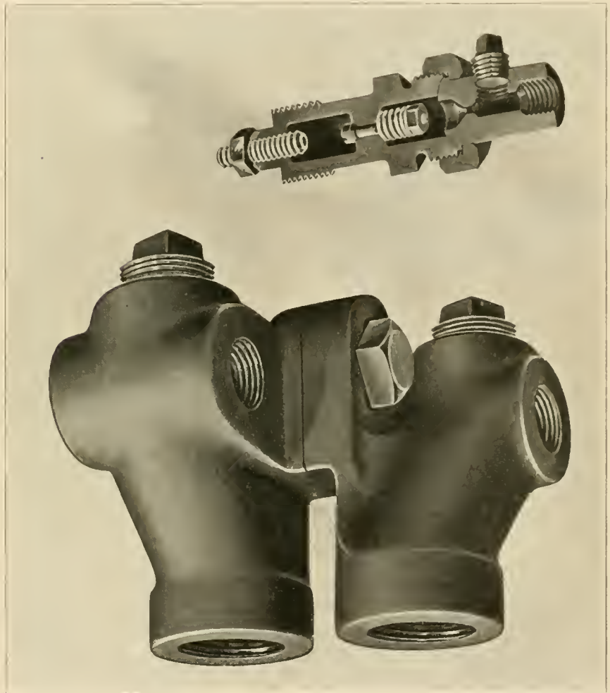
NEW CLASS E SANDER TRAP.
